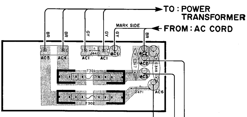
Main Circuit Board (3)
