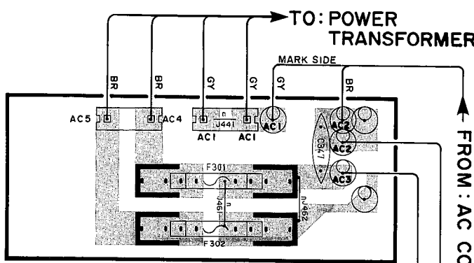
Main Circuit Board (3)
